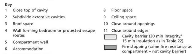
Figure 6-2 Figure 35 of BS 9999 – Provisions for cavity barriers
